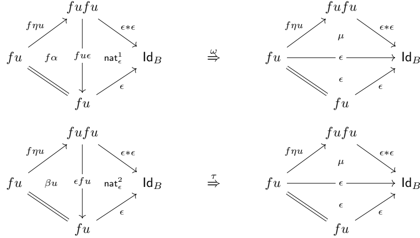
FIGURE 5. The 3-simplices in a half-adjoint diagrammatic adjunction
