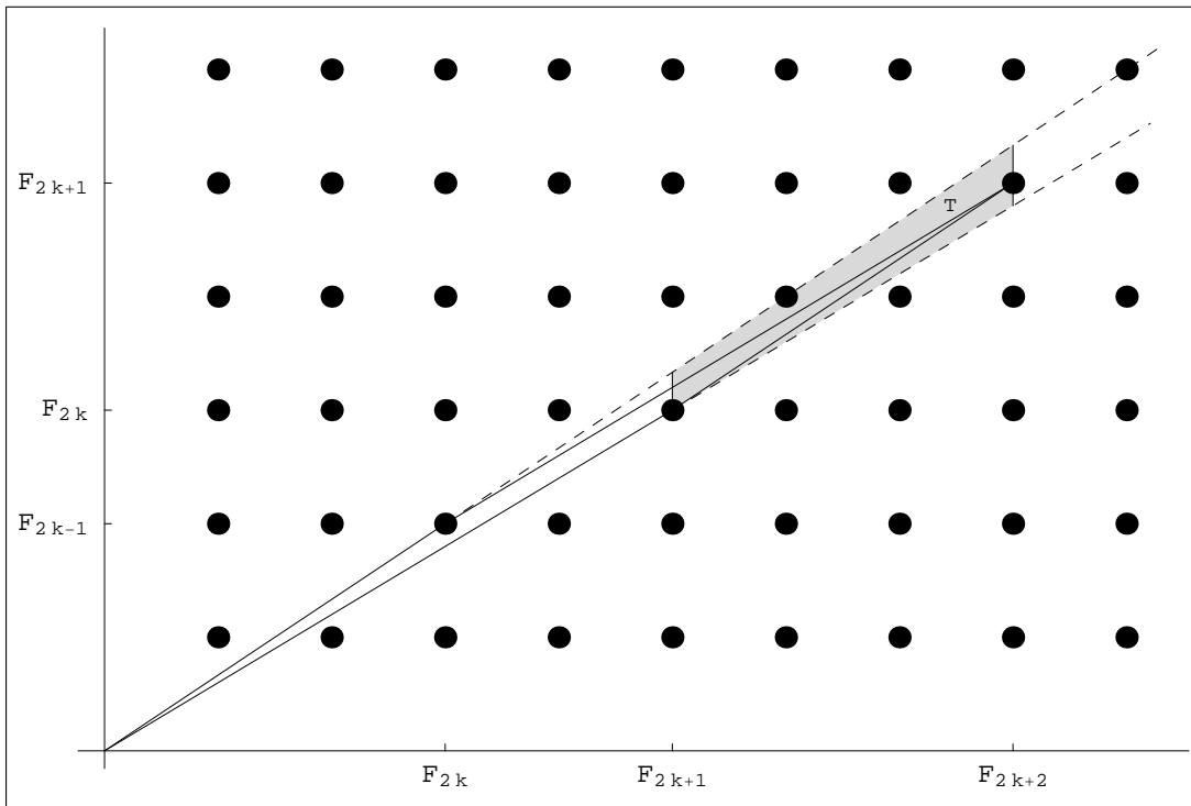
FIGURE 2. The region T
