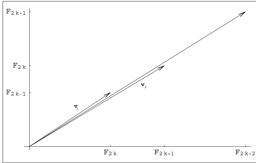
FIGURE 1. Ratios of consecutive Fibonacci numbers
